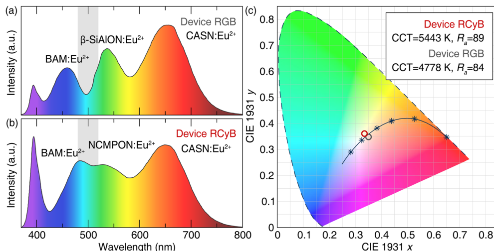
Fig. 8 The emission spectrum of a device constructed of (a) a red-green-blue (RGB) based white pc-LED made using \text{BaMgAl}_{10}\text{O}_{17}:\text{Eu}^{2+} ( \text{BAM}:\text{Eu}^{2+} ), \beta\text{-SiAlON}:\text{Eu}^{2+} , and \text{CaAlSiN}_3:\text{Eu}^{2+} ( \text{CASN}:\text{Eu}^{2+} ), and (b) a red-cyan-blue (RCyB) based white pc-LED made using \text{BAM}:\text{Eu}^{2+} , (\text{Na}_{13.57}\text{Ca}_{17.43})_{0.995}\text{Eu}_{0.155}\text{Mg}_5(\text{PO}_{3.75}\text{N}_{0.25})_{18} ( \text{NCMPON}:\text{Eu}^{2+} ), and \text{CaAlSiN}_3:\text{Eu}^{2+} with 395 nm LED. The gray area reflects cyan gap (480 nm to 520 nm) (c) The CIE coordinates of these devices demonstrate the production of daylight quality white light.
