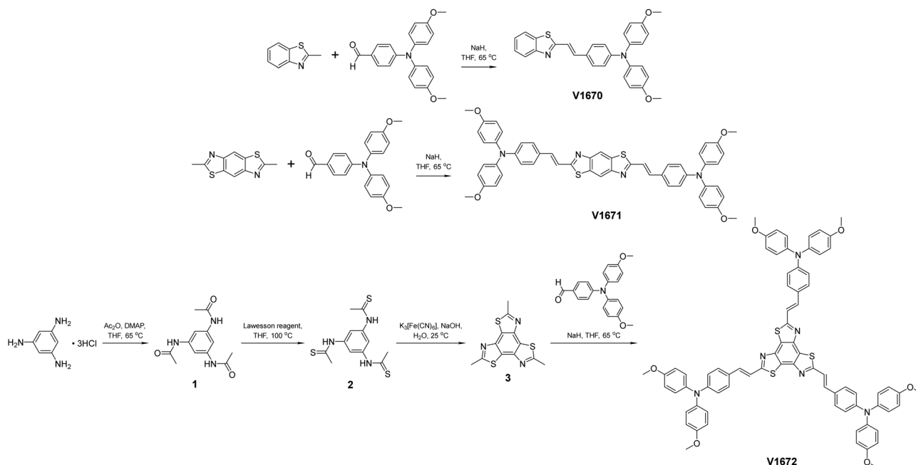
Fig. 1 Synthesis of target compounds V1670 , V1671 , and V1672 .
