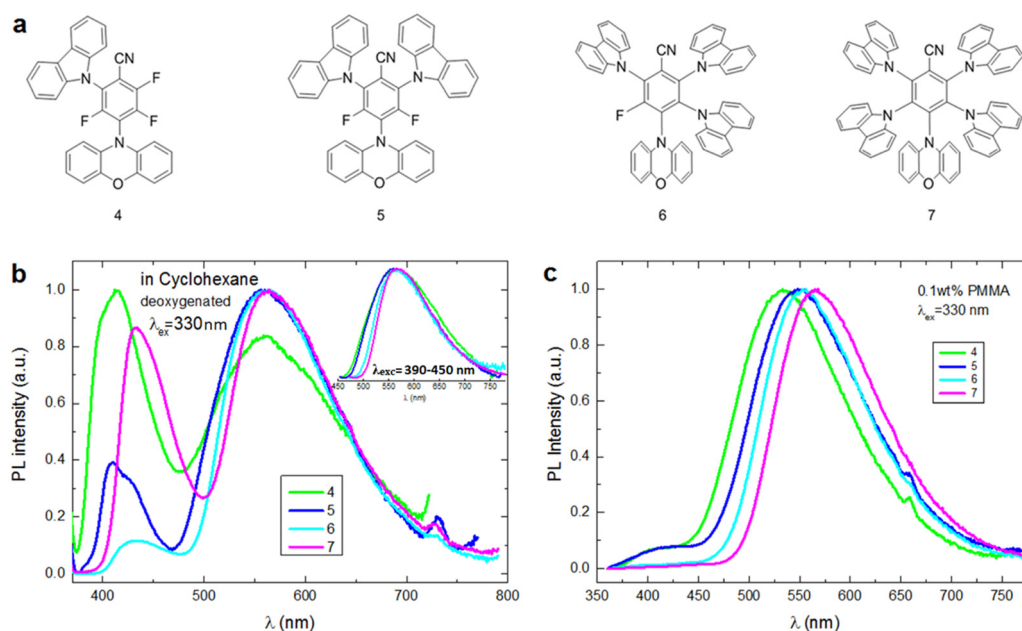
Fig. 1 (a) Molecular structures of the molecules studied. (b) Normalized photoluminescence spectra of 4–7 in cyclohexane (10 −5 M). Inset: Normalized photoluminescence spectra of 4–7 in cyclohexane (10 −5 M) excited on the lower energy CT band, λ exc = 390–450 nm. (c) Normalized photoluminescence spectra of 4–7 in PMMA.
