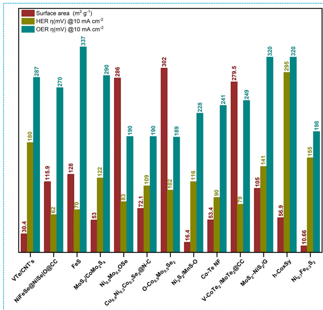
Fig. 8 The summary of the BET surface area, HER, and OER overpotential at 10 \text{ mA cm}^{-2} of the various porous metal chalcogenides. The data were initially reported as follows: VTe/CNTs, 180 NiFeSe@NiSe/O@CC, 181 Ni 0.5 Mo 0.5 OSe, 104 MoS 2 /CoMo 2 S 4 , 182 Cu 0.4 Ni 0.3 Co 0.3 Se 2 @N-C, 103 O-Co 0.5 Mo 0.5 Se 2 , 107 Ni 3 S 2 /MnS-O, 159 CoTe NF, 110 V-CoTe 2 /MoTe 2 @CC, 113 MoS 2 -NiS 2 /G, 138 h-Co x S y , 161 Ni 0.7 Fe 0.3 S 2 . 22
