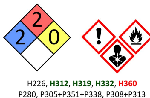
Chart 1 Summary of DMF hazards, NFW 704 safety square, warning symbols and hazard statements. Hazard statements are colour-coded according to their CHEM21 classification.
