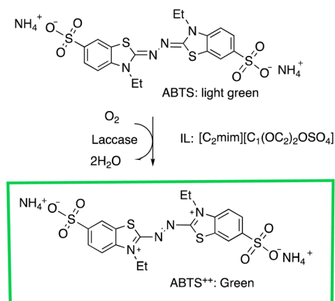
Fig. 7 Additive effect of an IL ( [C_2\text{mim}][C_1(\text{OC}_2)_2\text{OSO}_4] ) on the laccase-mediated oxidation of ABTS. 91
