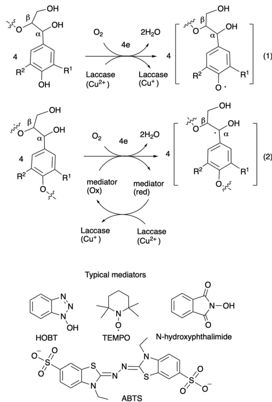
Fig. 3 Laccase-mediated oxidation. 17,29,76–78
