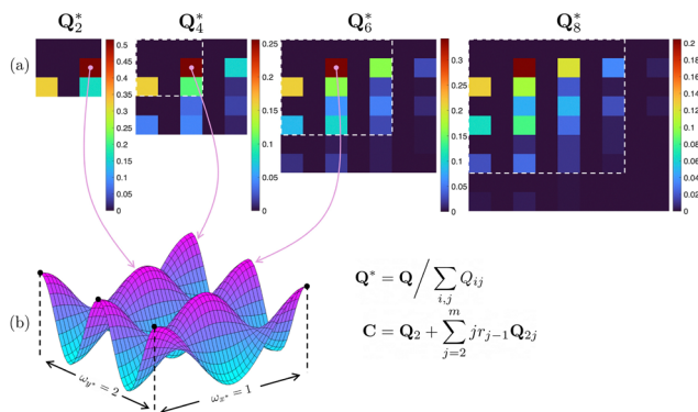
Fig. 2 (a) Visualization of \mathbf{Q}^* -matrix where the colour represents the weight of each wrinkling modes in a \mathbf{Q} -matrix. The dash line encircles the location of previous \mathbf{Q}^* -matrix. The index (i, j) of each \mathbf{Q}^* -matrix corresponds to a unique wrinkling mode with \omega_{x^*} = (i - 1) and \omega_{y^*} = (j - 1) . For example, the (2, 3) component of each \mathbf{Q}^* -matrix represents a wrinkling mode \cos 2\pi(2 - 1)x^* \cos 2\pi(3 - 1)y^* described by (b).
