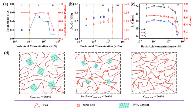
Fig. 24 (a) Total strain at point A and total strain of the elastic plateau at different c_{BA} , (b) median D_{res}/2\pi and \sigma/2\pi as a function of c_{BA} , (c) change in L (long period), d_c , and d_b (the distance between two lamellae) as a function of c_{BA} and (d) mathematical model of the PVA film (gel state) in the presence of BA. The destruction of the crystalline lamellae is also illustrated. Reprinted with permission from ref. 170; copyright 2024, the American Chemical Society.
