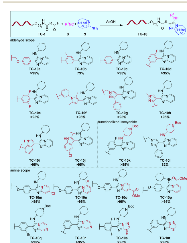
Fig. 5 Scope of the Groebeke–Blackburn–Bienaymé three-component reaction on 10mer TC-DNA. Reaction conditions: TC-1 (3 nmol) and copolymer (90 nmol) and heteroaromatic amine 9 (6 \mu mol) in MeOH/CHCl 3 (80 \mu L; 7:1, v/v) for 6 h at rt. Addition of isocyanide 3 (6 \mu mol) and acetic acid (0.8 \mu L; c = 1 vol%). The reaction was run for 16 h at 25 °C.
