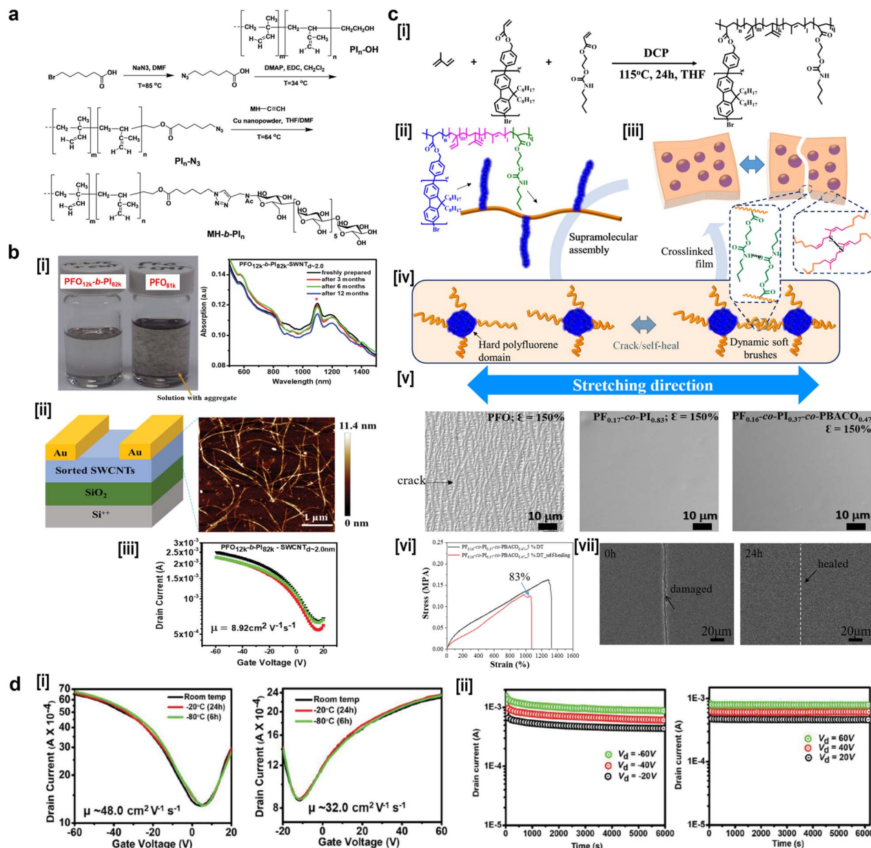
Fig. 8 (a) The synthesis routes of MH-b-PI n block copolymers for stretchable resistive memory device application. (b) SWCNTs-thin film transistor fabrication: (i) stability and dispersion study based on photograph image and UV-spectra, (ii) schematic of BGTC transistor configuration and AFM image of SWCNTs sorted by PFO 12K -b-PI 82K , and (iii) I D -V G transfer curve of the device using PFO 12K -b-PI 82K -dispersed sc-SWCNTs (diameter ≤ 2.0 nm) as the semiconducting layer. (c) Molecular design of the intrinsically elastic and self-healing luminescent PF x -co-PI y -co-PBACO z : (i) synthetic scheme; (ii) branched copolymer with soft PI-co-PBACO backbone (blue) and rigid PF branches (orange); (iii) self-assembled into a two-phase nanostructure; (iv) elasticity tuning via DT cross-linking (gray spheres) and hydrogen bonding (dotted lines); (v) OM images of the PF, PF 0.17 -co-PI 0.83 , and PF 0.16 -co-PI 0.37 -co-PBACO 0.47 thin films under 150% strain, and (vi) investigation of RT self-healing performance of the PF 0.16 -co-PI 0.37 -co-PBACO 0.47 film based on tensile test and SEM images before (0 h) and after (24 h) self-healing. (d) The (i) I D -V G transfer curves and (ii) retention stability of p-type and n-type PFO 0.16 -co-PI 0.36 -co-PBACO 0.48 -sc-SWCNTs respectively, where the retention tests were performed at gate voltages of ±60 V. Reprinted with permission from ref. 19. copyright 2017 John Wiley & Sons., ref. 134 copyright 2021 John Wiley & Sons, ref. 62 copyright 2022 American Chemical Society, ref. 139 copyright 2022 John Wiley & Sons.
