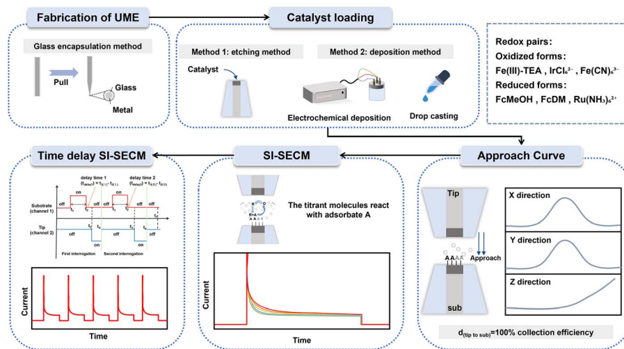
Fig. 3 Schematic illustration of the typical experimental procedure for SI-SEC.
