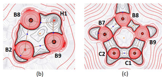
Fig. 8 (a) Selected NBO of 5 showing the 3c–2e interaction of B8–H1–B9 (isocontour values: \pm 0.045 [ \text{e bohr}^{-3} ] ^{1/2} ). Contour-line diagram of the Laplacian of the electron density along (b) B8–H1–B9 and (c) B7–B8–B9 planes in 5 .
