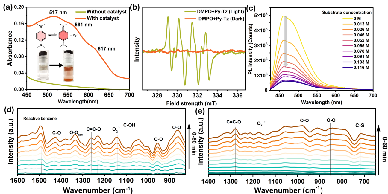
Fig. 3 (a) UV-vis spectra of TMPD radical cation formed by Py-Tz COF in the presence of light and O_2 . (b) EPR spectra of DMPO- O_2^{\cdot-} formed by Py-Tz COF in the presence of light. (c) Photoluminescence quenching experiment of Py-Tz COF in THF dispersion by varying concentrations of N,N -dimethylaniline. In situ DRIFT studies demonstrate the appearance of new peaks, showing the progression of (d) hydroxylation reaction and (e) thiocyanation reaction.
