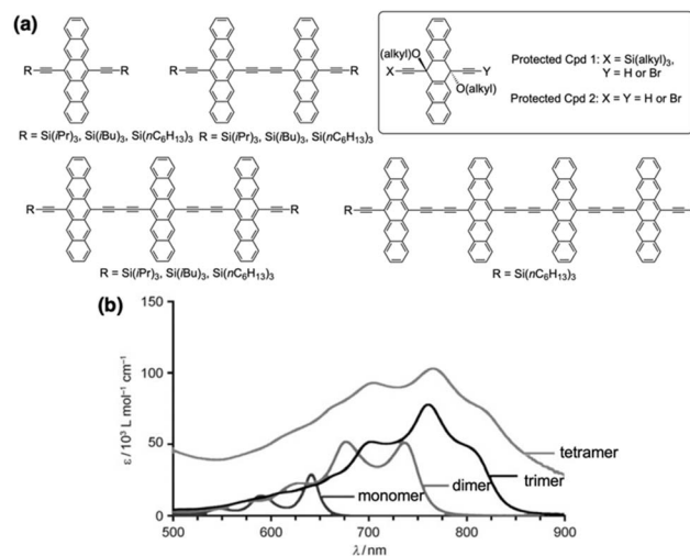
Fig. 39 (a) Pentacene oligomers employed in this study. Protected building blocks are also shown. (b) Absorption spectra of oligomers. R = \text{Si}(\text{nC}_6\text{H}_{13})_3 . Adapted with permission from ref. 147. Copyright 2012 Wiley.
