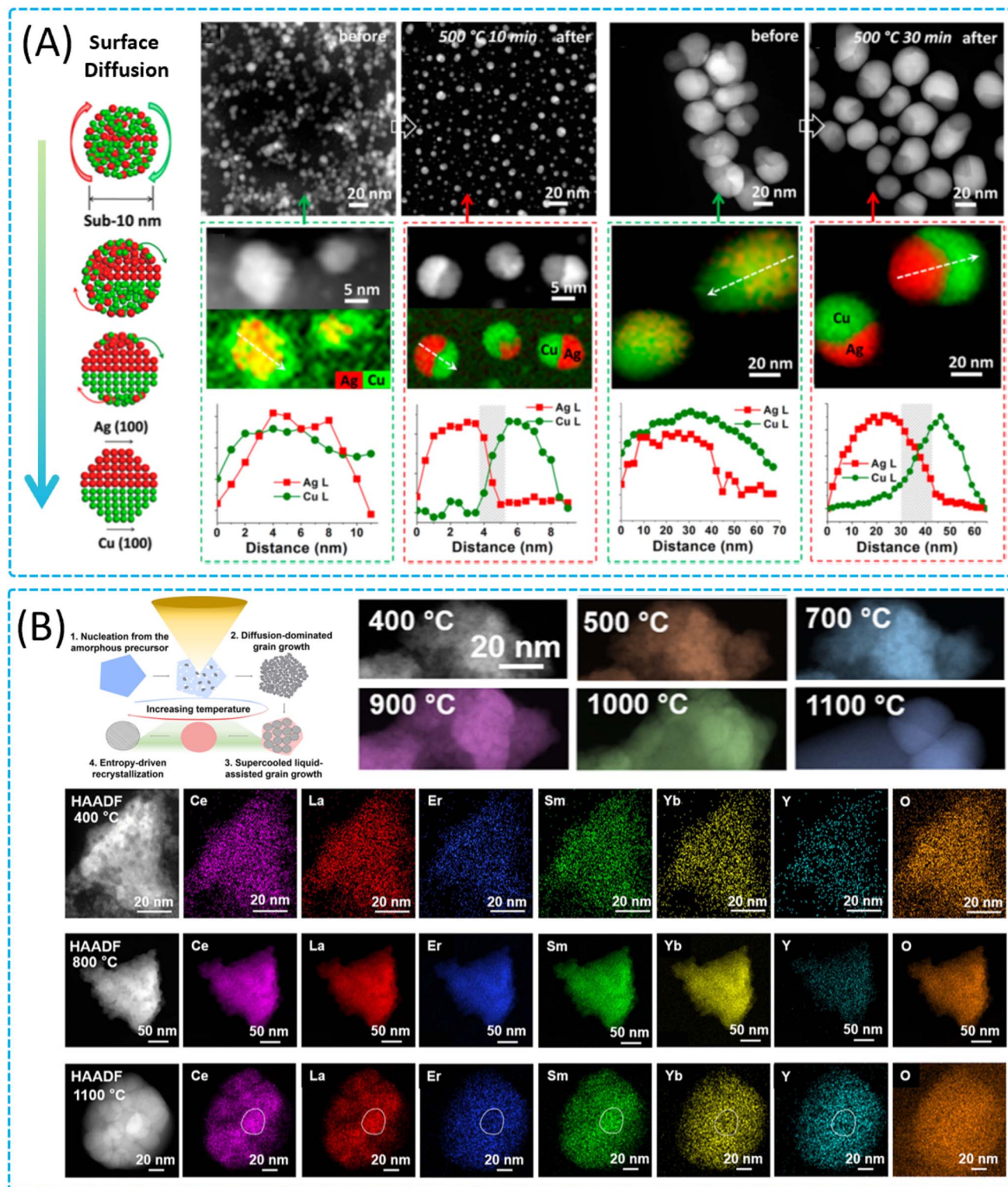
Fig. 4 Phase transition of 0D nanomaterials in solid-state interactions. (A) Schematic representations of the reasonable atomic motion in sub-10 nm CuAg nanoparticles during annealing to form a Cu(100)/Ag(100) heterointerface, and STEM-HAADF images of CuAg nanoparticles before and after annealing under vacuum at 500 °C for 10 min. The corresponding high-magnification STEM-HAADF images and EDS elemental maps. Reproduced with permission. 32 Copyright 2019, American Chemical Society. (B) Schematic representations of the HEFO from an amorphous precursor and characterization of the structures and compositions of high-entropy fluorite oxides at different temperatures. Reproduced with permission. 97 Copyright 2022, American Chemical Society.
