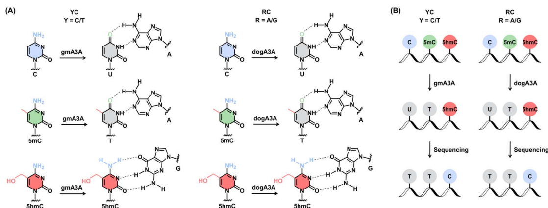
Fig. 2 Schematic illustration of the OMA-seq method. (A) Deamination patterns at YC and RC sites. C and 5mC are converted to U and T, respectively, by gmaA3A (for YC sites) and dogA3A (for RC sites), while 5hmC remains resistant to deamination. As a result, U and T base pair with A, whereas 5hmC base pairs with G. (B) Sequencing results after treatment with gmaA3A (for YC sites) and dogA3A (for RC sites). C and 5mC are deaminated and read as T, whereas 5hmC is not deaminated and retains its original base pairing. By combining gmaA3A and dogA3A, OMA-seq enables site-specific and quantitative detection of 5hmC in diverse sequence contexts.
