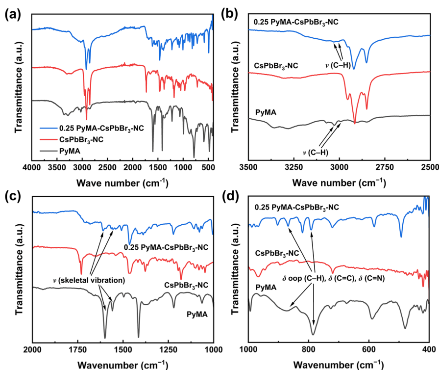
Fig. 5 (a) FT-IR spectra of PyMA, CspBr 3 -NC, and 0.25 PyMA-CspBr 3 -NC. The zoomed-in FT-IR spectra in the (b) 2500–3500 cm -1 , (c) 1000–2000 cm -1 , and (d) 400–1000 cm -1 regions.
