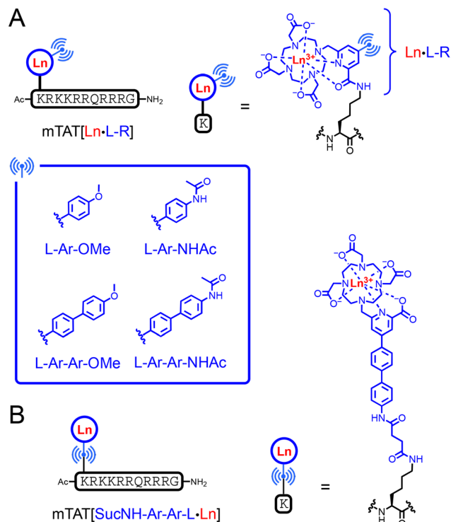
Fig. 2 Chemical structures of (A) mTAT[Ln \cdot L-R] conjugates ( R = Ar-OMe , Ar-NHAc , Ar-Ar-OMe and Ar-Ar-NHAc ; Ln = Eu^{3+} or Gd^{3+} ) and (B) the mTAT[SucNHArArL \cdot Ln] conjugate.
