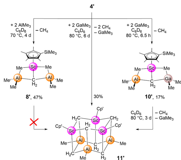
Scheme 5 Reactions of \text{Cp}'\text{Sc}(\text{AlMe}_4)\text{Me} ( 4' ) with \text{AlMe}_3 or \text{GaMe}_3 to form \text{Sc}/\text{Al}_2 methylidene 8' or mixed \text{Sc}/\text{Al}/\text{Ga} methylidene 10' and its reaction to [\text{Cp}'\text{Sc}(\text{CH}_2)_2\text{AlMe}_3] ( 11' ).
