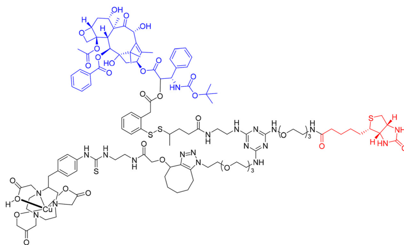
Fig. 16 Chemical structures of compounds 23, 24 and 25.
