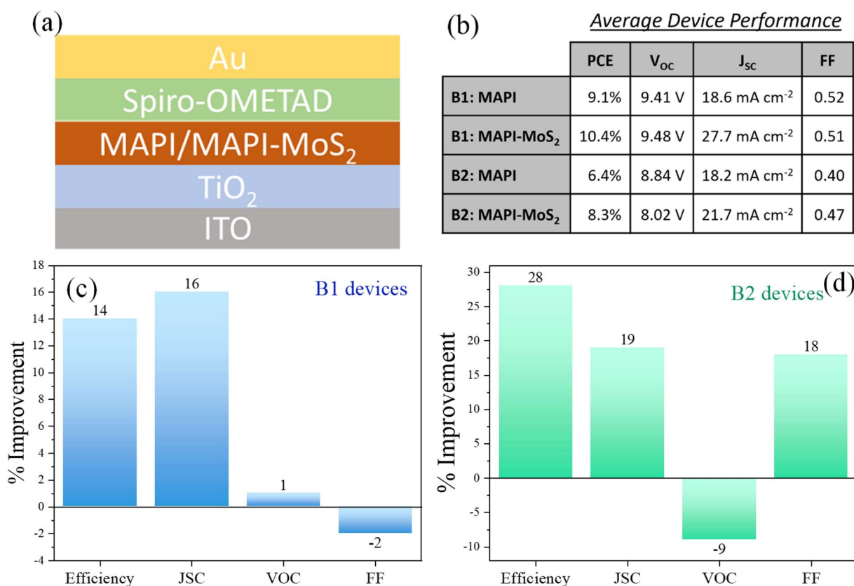
Fig. 5 (a) Diagram of the device structure. (b) Average device performance parameters. (c and d) Changes in performance parameter of the MAPI–MoS 2 devices with respect to the corresponding MAPI-only devices for the two sets of solar cells prepared in different laboratories (B1 and B2): power conversion efficiency (PCE), open circuit voltage ( V_{OC} ), short circuit current density ( J_{SC} ) and fill factor (FF).
