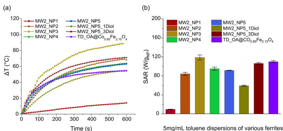
Fig. 7 Heating efficiency of particles synthesized with the MW2 method: (a) temperature variation as a function of time and (b) SAR values measured for 5 mg mL -1 of magnetic cobalt ferrite particle dispersion.
