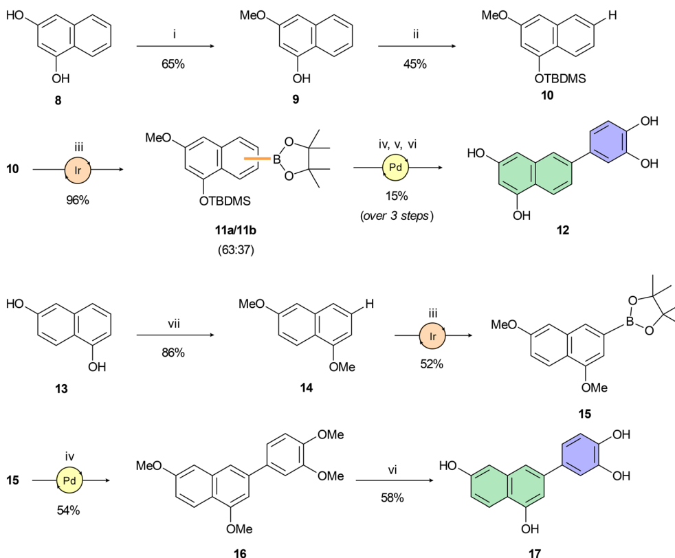
Scheme 2 Reagents and reaction conditions: (i) 4 M HCl (1,4-dioxane), MeOH, 0 °C \rightarrow r.t., 24 h; (ii) TBDMSCl, imidazole, THF, 0 °C \rightarrow r.t., 16 h; (iii) B_2(p\text{in})_2 , [Ir(COD)OMe]_2 (4 mol%), n -hexane, 100 °C, 16–72 h; (iv) 4-bromoveratrole, SPhos Pd G2 (10 mol%), K_2CO_3 , THF/ H_2O (25:1), 100 °C, 16 h; (v) TBAF, THF, 0 °C, 2 h; (vi) BBr_3 , DCM, 0 °C \rightarrow r.t., 2 h; (vii) MeI, K_2CO_3 , DMF, r.t., 18 h.
