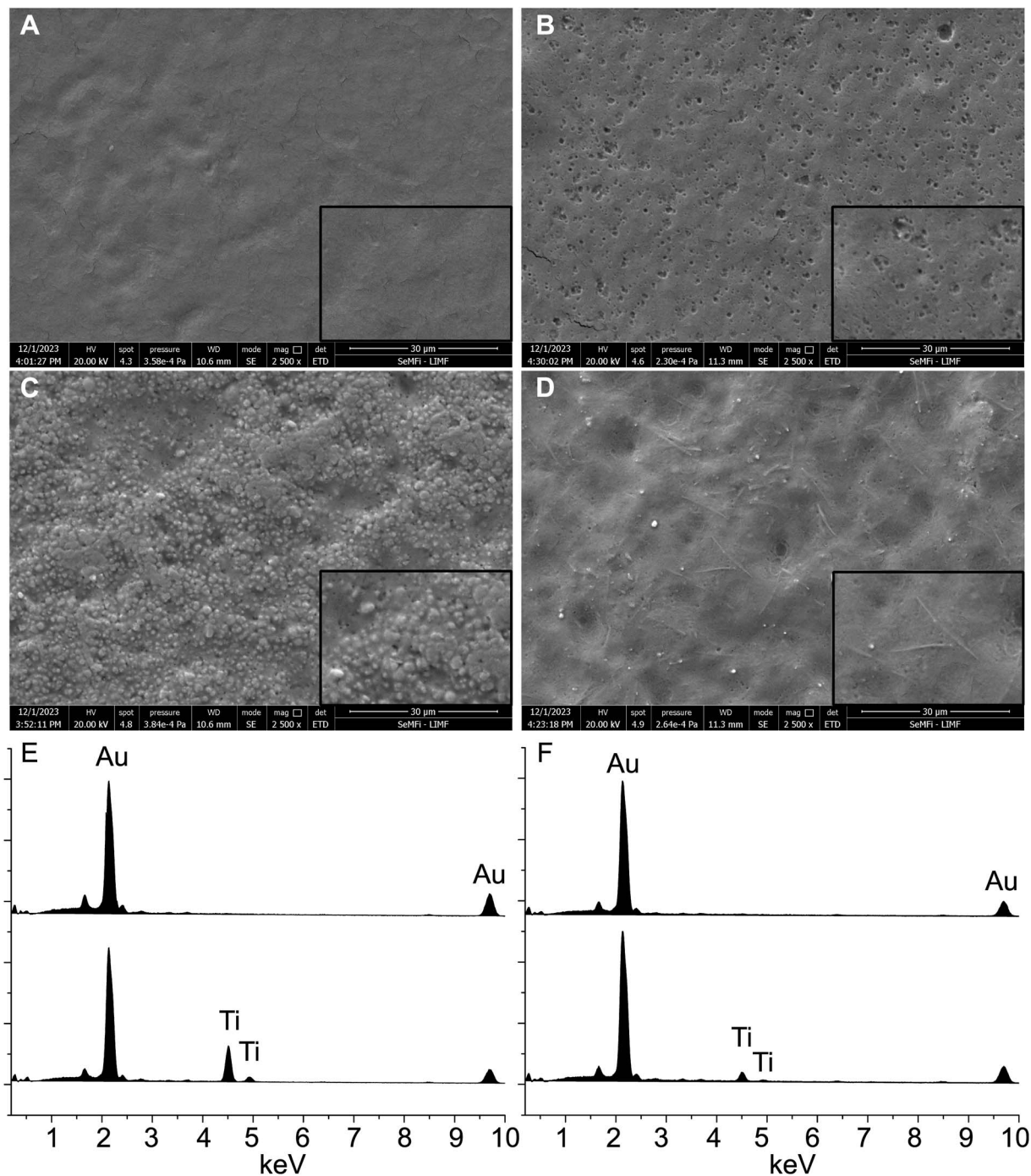
Fig. 5 SEM micrographs of the upper surface (A and B) and lower surface (C and D) of films reinforced with nanospheres (A and C) or nanotubes (B and D). Scale bar 30 \mu\text{m} . Inset 10 \mu\text{m} . EDS signals from films reinforced with nanospheres (E) or nanotubes (F). Upper trace corresponds to the upper surface and lower trace to the lower surface. Scale bar 30 \mu\text{m} .
