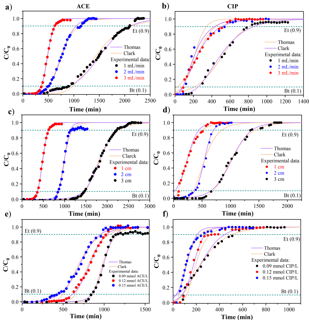
Fig. 4 Adsorption in continuous systems a) and b) effect of flow on breakthrough curves (conditions: a) 1 cm, 0.09 mmol ACE per L; b) 1 cm, 0.09 mmol CIP per L. c) and d) Effect of bed height on breakthrough curves under the following (conditions: c) 3 mL min -1 , 0.09 mmol ACE per L; d) 2 mL min -1 , 0.09 mmol CIP per L. e) and f) Effect of feed concentration on breakthrough curves (conditions: e) 2 cm, 3 mL min -1 ; f) 1 cm, 2 mL min -1 ). E_t : exhaustion time = 0.9, B_t : breakthrough time = 0.1.
