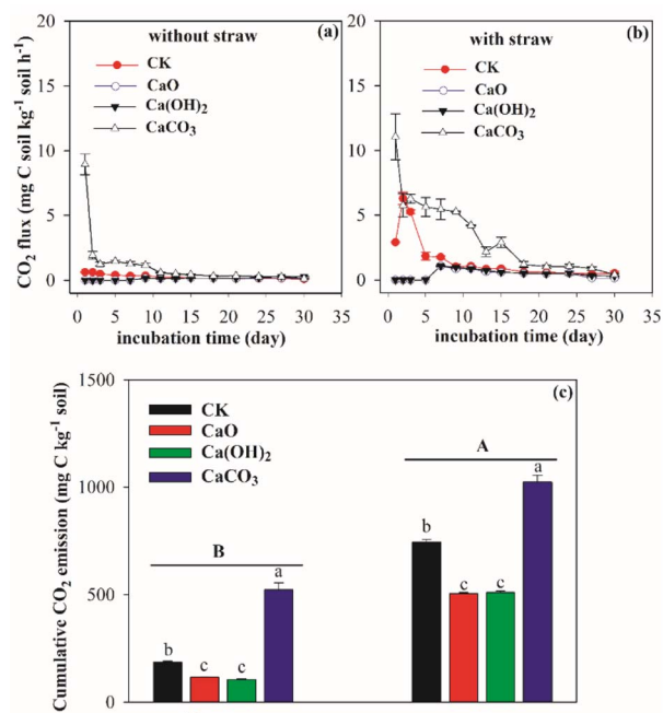
Fig. 2 CO 2 fluxes and (a and b) and cumulative emissions (c) from different treatments over the 30-day incubation period. Error bars represent standard errors of the mean values ( n = 3 ). Different uppercase letters and lowercase letters indicated the significant difference between straw and no straw treatments, and the difference among different lime materials treatments ( P < 0.05 ), respectively.
