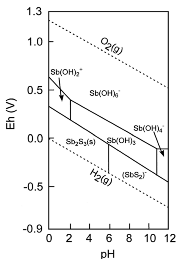
Fig. 1 Eh–pH diagram of antimony in the Sb–S– \text{H}_2\text{O} system at a dissolved antimony concentration of 10^{-8} \text{ mol L}^{-1} and a dissolved sulfur concentration of 10^{-3} \text{ mol L}^{-1} (reproduced from Filella et al. , 2002; with permission from Elsevier). 10
