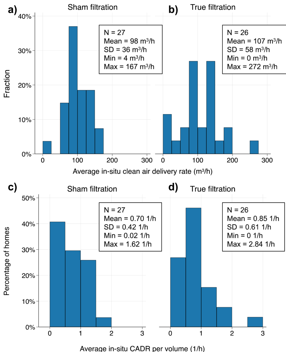
Fig. 2 Interim analysis of (a and b) time-averaged in situ CADR ( \text{m}^3 \text{ h}^{-1} ) and (c and d) CADR divided by house volume (CADR/V, 1/\text{h} ) for smoke-sized particles delivered in the 53 homes with interim visits to date, split by sham and true filtration groups. Estimates of CADR and CADR/V for sham filtration group assume what the CADR would be if true filtration was used for direct comparison to true filtration group.
