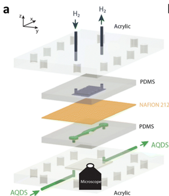
Fig. 14 Microfluidic flow cell compatible with electrochemistry and confocal microscopy. (a) Scheme of the individual components. (b) Photographs of the assembled cell from above (top) and below (bottom). The working electrode ( 3 \times 6 \text{ mm}^2 ) is visible in the center of the bottom image. For the bottom picture a working electrode made of gold was used to ensure visibility against the counter electrode in the background. 160 Reproduced with permission. Copyright 2024, RSC Publication.
