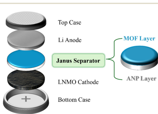
Fig. 1 Schematic representation of the cell configuration with the Janus separator.
