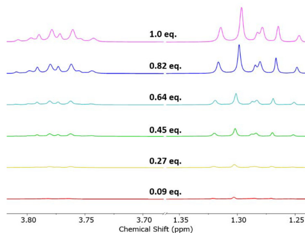
Fig. 7 Stacked plot of 1 H NMR spectra (DMSO-d 6 ) following the portionwise addition of Na(Et 2 dtc) to Na[AuCl 4 ]. The majority product is [Au(Et 2 dtc) 2 ] + and the minority product is [AuCl 2 (Et 2 dtc)].
