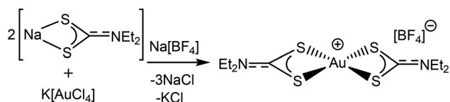
Scheme 3 Synthesis of [Au(Et 2 dtc) 2 ][BF 4 ] (reaction conducted in acetone).
