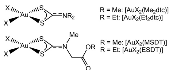
Fig. 1 A selection of “[AuX 2 (dte)]” complexes which have demonstrated anti-cancer activity (X = Cl, Br).
