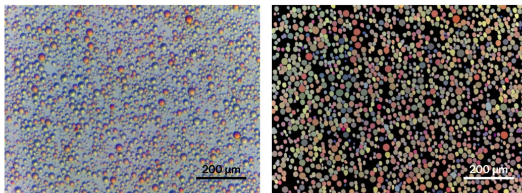
Fig. 4 Yellow Ce(IV) and red ferroin(II) microdroplets observed via optical microscopy along with blue ferroin(III) product (left). Computational segmentation with representative RGB sampled from the centre of each region (right).
