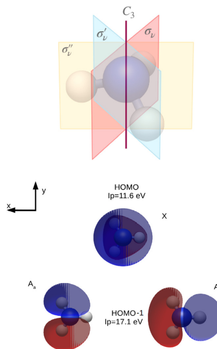
Fig. 6 Representation of the \text{NH}_3 molecule with the reflection planes and the C_3 rotational axis, and \text{NH}_3 HF occupied MOs studied in this work.
