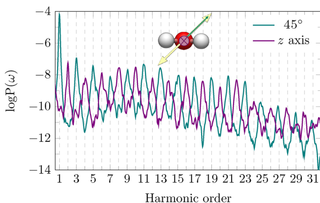
Fig. 5 Total HHG spectra of \text{H}_2\text{O} obtained with pulse polarisation of 45^\circ in the xy plane, i.e. the configuration (d) in Fig. 2. In green the spectrum recorded in the same direction of pulse polarisation, in violet the spectrum detected along the z axis.
