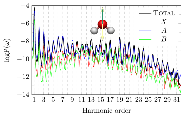
Fig. 4 Total and partial HHG spectra of \text{H}_2\text{O} , with pulse polarisation parallel to the principal axis ( z axis). This system corresponds to the configuration (c) of Fig. 2. The yellow double arrow represents the pulse polarisation, while a green arrow represents the direction of detection of the HHG signal.
