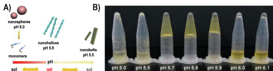
Fig. 27 Schematic illustration for the ultra-pH-sensitive of Fc-L-Phe-L-Phe hydrogel (A) and photographic images showing the self-assembly behavior of 2 mg mL -1 Fc-L-Phe-L-Phe in 10% 2-propanol/90% H 2 O at phosphate buffer (0.1 M) with different pH values (B). Reproduced and adapted from ref. 240 with permission from Elsevier, copyright 2020.
