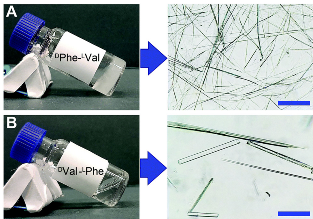
Fig. 25 Photographs and optical microscopy images of (A) D-Phe-L-Val and (B) D-Val-L-Phe in PBS at concentrations above their solubility. Scale bar = 100 \mu\text{m} . Reproduced and adapted from ref. 202 with permission from Royal Society of Chemistry, copyright 2022.
