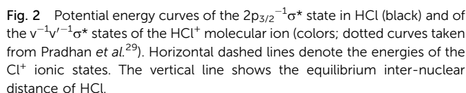
ences between the asymptotic states are not entirely reliable. To improve this, we assign each molecular state its dissociation limit using the Wigner-Witmer rules. 45 As indicated in the last column of Table 1, the limits correspond to excited states of the \text{Cl}^+ ion with two 3s and/or 3p vacancies. Our PECs are shifted vertically to match the energy differences of the corresponding atomic states, taken from ref. 46, in the dissociation limit. The resulting PECs are shown in Fig. 2.
