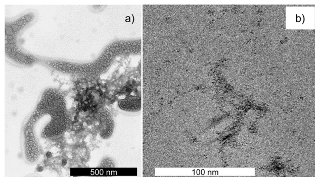
Fig. 9 Experimental investigation of LLPS in oxides a) cryo-TEM prior to boehmite crystallization, frozen ca. 10 ms after reaction. Adapted with permission from Haberkorn et al. 40 Copyright 2003 Elsevier. Bubbling is induced by the electron beam to demonstrate the difference between the dense liquid precursor and solid-state amorphous particles. b) Cryo-TEM prior to magnetite crystallization, aliquot of a dilute HCl solution titrated with a FeCl 3 solution. Adapted with permission from Scheck et al. 41 Copyright 2016 American Chemical Society. The granular structure is assigned to pre-nucleation clusters.
