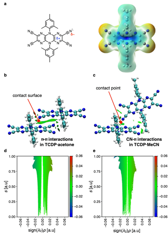
Fig. 10 (a) Electrostatic potential map of TCDP . (b) NCI plots of \pi - \pi interactions in TCDP-acetone and (c) \text{CN}-\pi interactions in TCDP-MeCN . An isosurface value of 0.3 a.u. was applied to the structure. (d and e) Plot of s vs. \text{sign}(\lambda_2)\rho for TCDP-acetone (d) and TCDP-MeCN (e). A large, negative value of \text{sign}(\lambda_2)\rho indicates an attractive interaction, while a large, positive value reflects strong non-bonding overlap.
