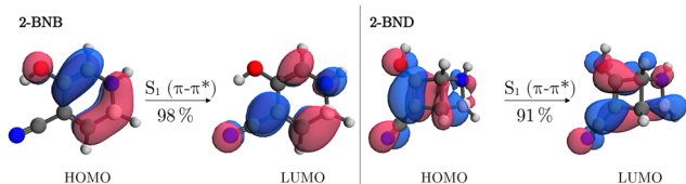
Fig. 5 Visualisation of the main orbital contributions of the first excited state of 2-BNB (left) and 2-BND (right) at the equilibrium geometry from TDDFT calculations. Depicted with an isovalue of 0.100.
