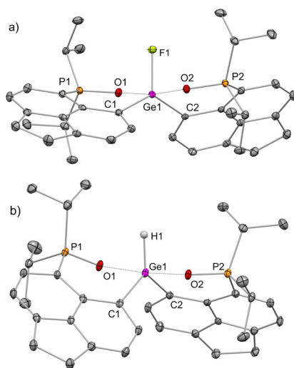
Fig. 4 Molecular structures of (A) 1 iPr PO-F and (B) 1 iPr PO-H in the solid state (thermal ellipsoids 35%, H atoms, triflate counter anions and solvent molecules are omitted for clarity). Selected bond lengths [Å] (a) Ge1-F1 = 1.746(2), Ge1-O1 = 1.971(2), P1-O1 = 1.524(2), Ge1-O2 = 1.990(2), P2-O2 = 1.525(2); (b) Ge1-H1 = 1.436(2), Ge1-O1 = 2.013(2), P1-O1 = 1.520(2), Ge1-O2 = 2.056(2), P2-O2 = 1.517(2).
