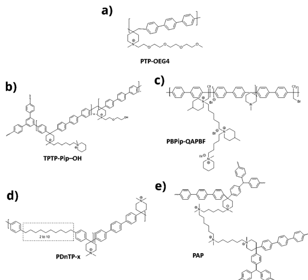
Fig. 16 Chemical structure of (a) PTP-OEG4, (b) TPTP-Pip-OH, (c) ether-free fluoropolymer PBIP-QAPBF, (d) poly(aryl-co-terphenyl piperidinium) based AEMs PDnTP-x and (e) poly(aryl piperidinium) (PAP) based anion exchange membranes.
