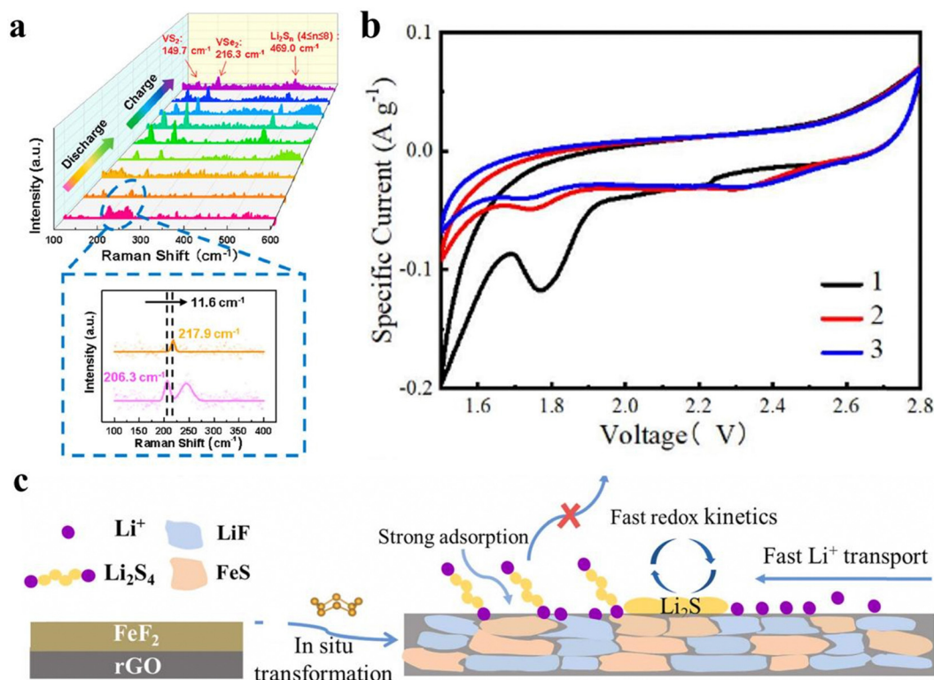
Fig. 5 (a) Operando Raman spectra at different discharge and charge states and the magnified view of the signal of \text{VS}_2 . Reproduced with permission from ref. 65 Copyright (2020) American Chemical Society. (b) Cyclic voltammetry curve of \text{FeF}_2/\text{rGO} cathode without sulfur. (c) Schematic diagram of the cathode catalytic conversion process during the cycle. Reproduced with permission from ref. 66 Copyright (2022) Elsevier.
