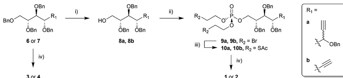
Scheme 2 Synthesis of target probes 1–4 . (i) ZnCl 2 , Ac 2 O, AcOH, 0 °C to rt; then K 2 CO 3 , MeOH, rt, 8a : 71% (dr 3:1), 8b : 68% over two steps. (ii) OP(OCH 2 CH 2 Br) 3 , Tf 2 O, pyridine, CH 2 Cl 2 , rt, 9a : 65% (dr 3:1), 9b : 57%. (iii) KSAC, pyridine, rt, 10a : quantitative (dr 3:1), 10b : quantitative. (iv) BCl 3 , CH 2 Cl 2 , –78 °C; then Ac 2 O, pyridine, rt, 1 : 31% (dr 7:1), 2 : 34%, 3 : 85% (dr 10:1), 4 : 57% over two steps.
