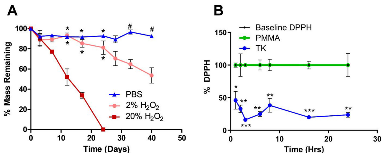
Fig. 3 (A) TK-ceramic scaffold degradation in aqueous and oxidative media ( n = 3 samples per treatment, *p < 0.05 comparing against 20% H_2O_2 , ^{\#}p < 0.05 comparing against 2% H_2O_2 ). TK samples also demonstrated potent antioxidative capacity by (B) significantly reducing the activity of DPPH radicals from their baseline and when compared against PMMA ( n = 3 samples per treatment, *p < 0.05 , **p < 0.01 , and ***p < 0.001 for TK vs. PMMA).
