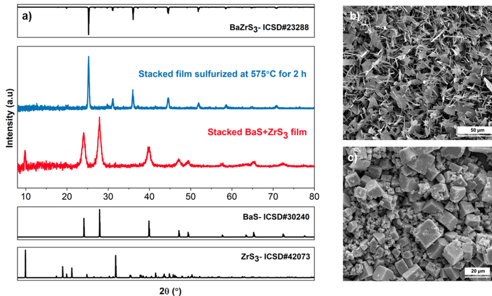
Fig. 5 (a) X-ray diffraction pattern showcasing the as-annealed stacked bilayer film of ZrS 3 and BaS before ampule sulfuration and the BaZrS 3 film after sulfuration. (b) SEM top-view image depicting the ZrS 3 film prepared from the ZrCl 4 –butylamine–CS 2 –pyridine solution chemistry. (c) SEM top-view image illustrating the BaZrS 3 film derived from the ZrS 3 –BaS bilayer stack.
