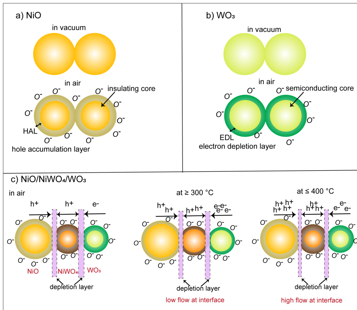
Fig. 5 (a) The effect of chemisorption on the conductance of NiO, (b) WO 3 and (c) NiO/NiWO 4 /WO 3 heterostructures.
