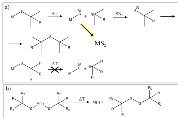
Fig. 4 (a) Thermal decomposition of thiolates and formation of \text{MS}_x nano-materials. Figure adapted from ref. 79 under Creative Commons Attribution licence CC BY 4.0 (b) redox reaction of thiolates and metals reported in ref. 86.
