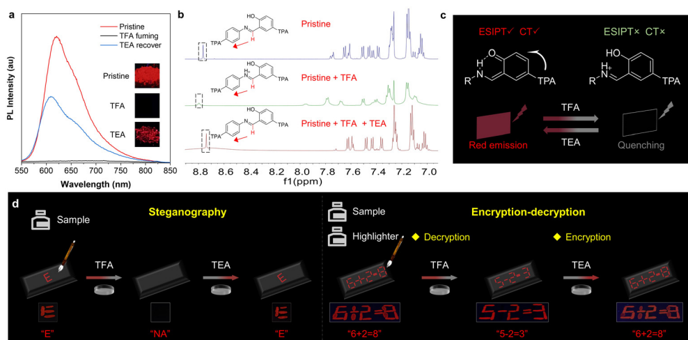
Fig. 5 (a) PL spectra of solid p,p -2TPA after different treatments. Inset: fluorescence photographs taken after the different treatments. (b) ^1\text{H} NMR spectra of p,p -2TPA before and after the addition of TFA and TEA in \text{CDCl}_3 . (c) Schematic diagram of the luminescence mechanism behind acid/base stimuli. (d) Application of stimuli-responsive p,p -2TPA for steganography and information encryption and decryption.
