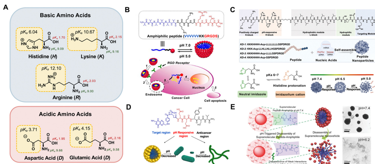
Fig. 2 (A) Structures of common basic and acidic amino acids, with their R-group side chain \text{pK}_a values highlighted and drawn in their charged configuration. The \text{pK}_a for N- and C-terminal groups are also shown for reference. (B) Schematic illustration of a pH-responsive micelle prepared from an amphiphilic peptide that assembles and disassembles to release anti-tumor drugs within cancer cells. Figure adapted from ref. 57 with permission from Elsevier © 2014. (C) Peptide designed to form pH-sensitive nanoparticles in complexation with nucleic acid payloads. The protonation equilibria and tautomeric forms of the imidazole side chain of histidine offer a pH triggered decomposition of the nanoparticles. Figure adapted from ref. 58 with permission from Royal Society of Chemistry © 2023. (D) Peptide sequence of prodrug FA-EEYSV-NH 2 and its properties pH-responsive assembled nanostructure. Figure adapted from ref. 59 with permission from American Chemical Society © 2021. (E) Scheme depicting the pH-responsive disassembly of complexed supramolecular amphiphiles, with TEM images showing the nanostructure at pH 7.4 and 6.2. Figure adapted from ref. 60 with permission from John Wiley and Sons © 2013.
