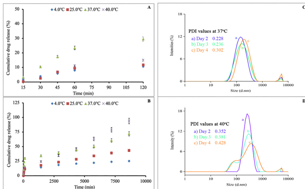
Fig. 5 Temperature-dependent drug release profile for (A) first 120 min and (B) 6 days. Size analysis of nanobubbles to assess thermal stability at (C) 37.0 °C and (D) 40.0 °C for (a) 2 days, 2880 min, (b) 3 days, 4320 min, and (c) 4 days, 5760 min.
