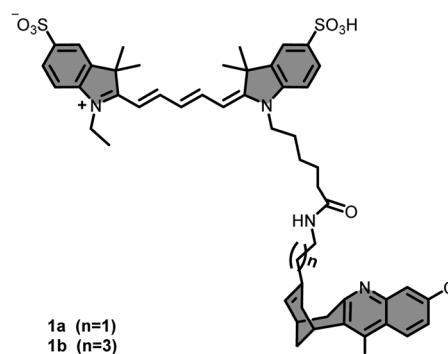
Fig. 5 Molecular structures of compound 1a and 1b .
